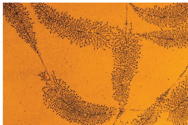
13.3 Under the electron microscope, DNA molecules undergoing transcription exhibit Christmas-tree-like structures. The trunk of each “Christmas tree” (a transcription unit) represents a DNA molecule; the tree branches (granular strings attached to the DNA) are RNA molecules that have been transcribed from the DNA. As the transcription apparatus moves down the DNA, transcribing more of the template, the RNA molecules become longer and longer. [Dr. Thomas Broker/Phototake.]
