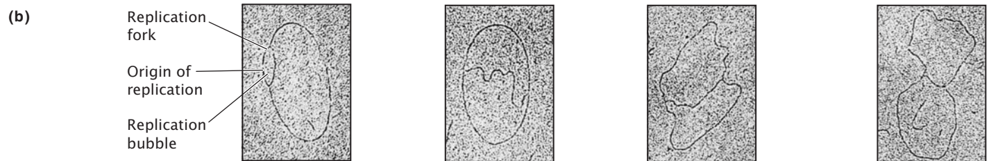
12.4 Theta replication is a type of replication common in E. coli and other organisms possessing circular DNA. [Electron micrographs from Bernard Hirt, L'Institut Suisse de Recherche Expérimentale sur le Cancer.]
