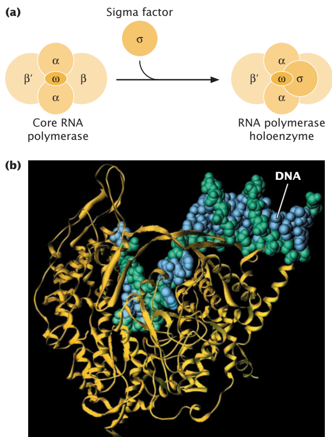
13.9 In bacterial RNA polymerase, the core enzyme consists of five subunits: two copies of alpha ( \alpha ), a single copy of beta ( \beta ), a single copy of beta prime ( \beta' ), and a single copy of omega ( \omega ). The core enzyme catalyzes the elongation of the RNA molecule by the addition of RNA nucleotides. (a) The sigma factor ( \sigma ) joins the core to form the holoenzyme, which is capable of binding to a promoter and initiating transcription. (b) The molecular model shows RNA polymerase (in yellow) binding DNA.
