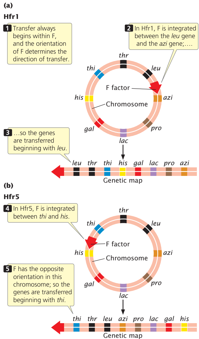
8.16 The orientation of the F factor in an Hfr strain determines the direction of gene transfer. Arrowheads indicate the origin and direction of transfer.
