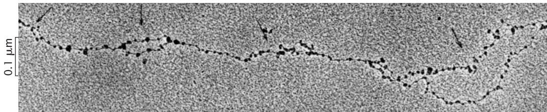
12.16 Nucleosomes are quickly assembled onto newly synthesized DNA. This electron micrograph of eukaryotic DNA in the process of replication clearly shows that newly replicated DNA is already covered with nucleosomes (dark circles). [Victoria Foe.]
