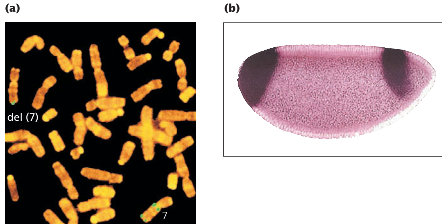
19.16 With in situ hybridization, DNA probes are used to determine the cellular or chromosomal location of a gene or its product. (a) A probe with green fluorescence is specific to chromosome 7, revealing a deletion on one copy of chromosome 7. (b) In situ hybridization is used to detect the presence of mRNA from the tailless gene in a Drosophila embryo. [Part a: Addenbrookes Hospital/Photo Researchers. Part b: Courtesy of L. Tsuda.]
