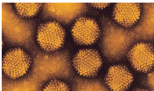
2.4 A virus is a simple replicative structure consisting of protein and nucleic acid. Adenoviruses are shown in the micrograph. [Micrograph by Hans Gelderblom/Visuals Unlimited.]
